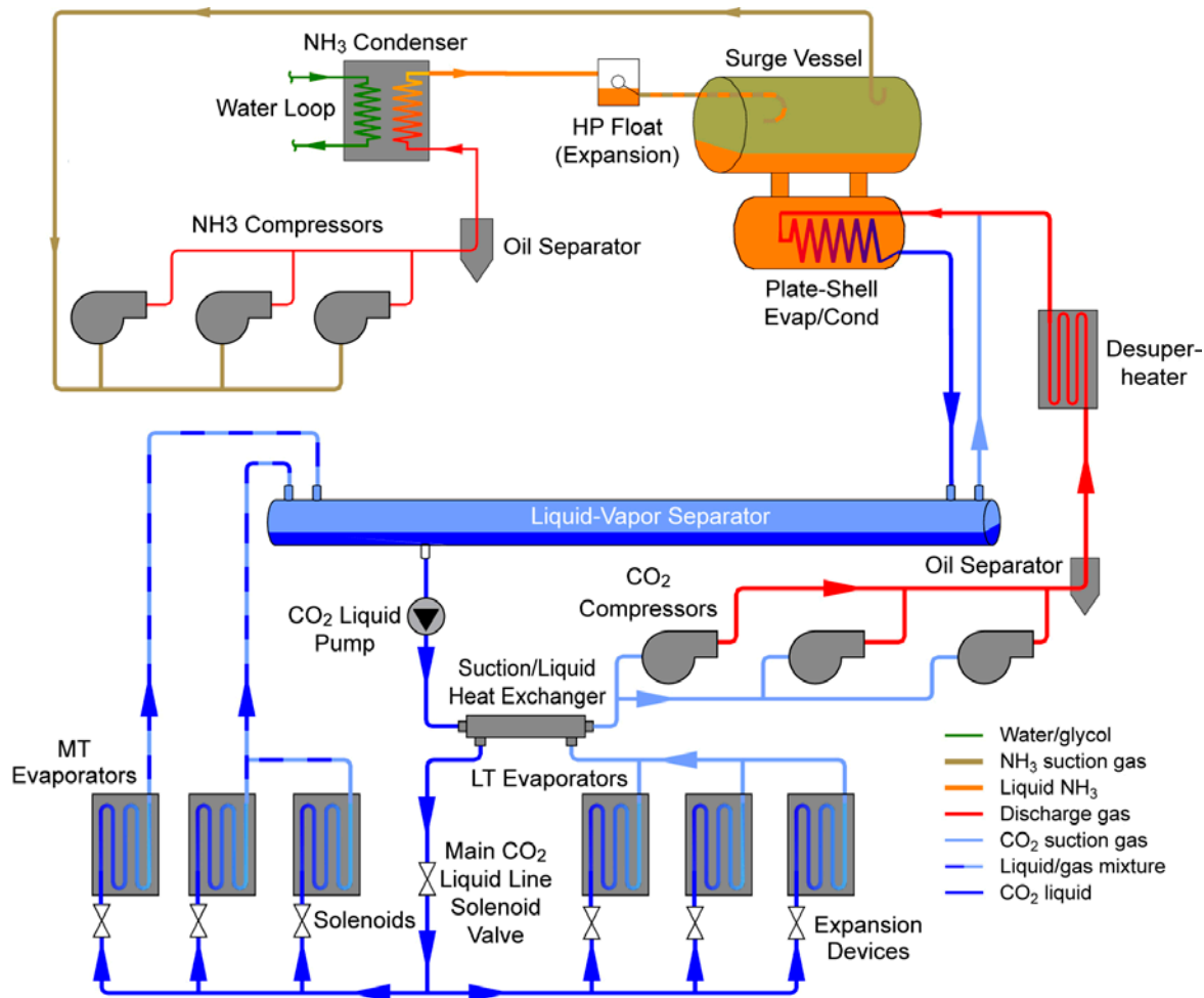
Figure 3-4. Combined MT pumped/LT DX \text{CO}_2 cascaded with \text{NH}_3 -flooded system
